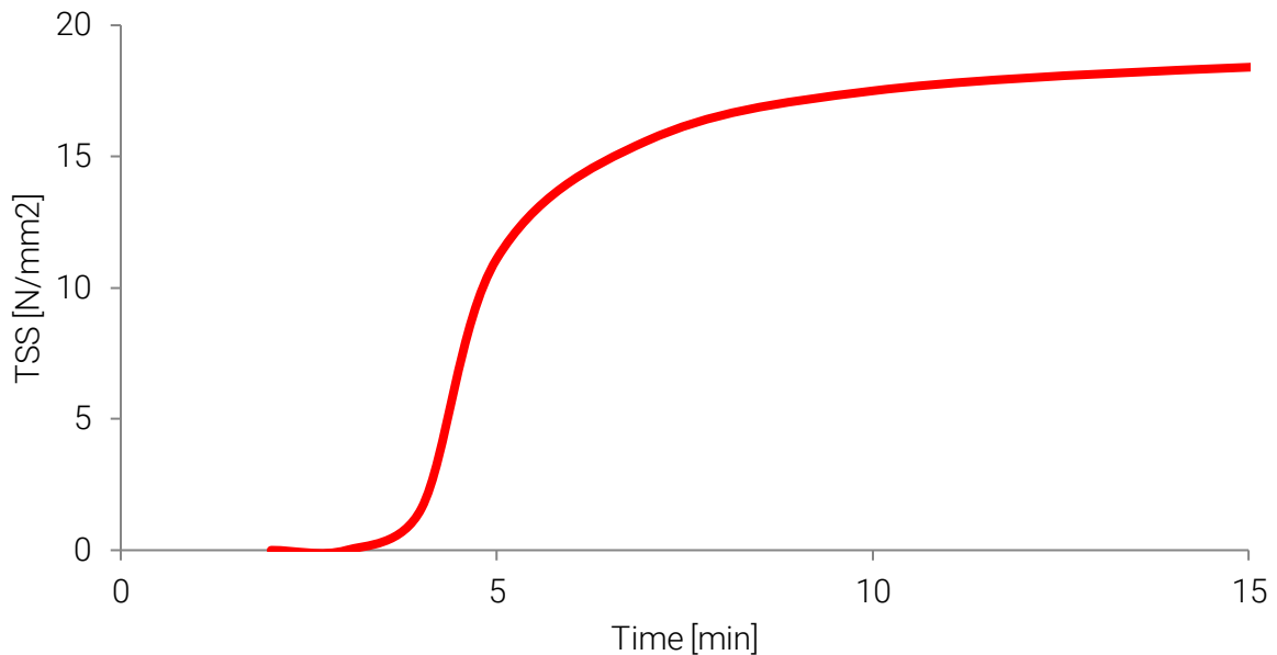
Tensile shear strength build-up on steel)
